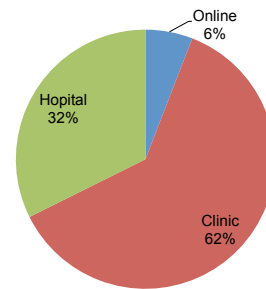
Figure 3: Sample size
