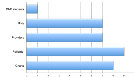
Figure 5: Statistics used
