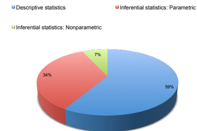
Figure 5: Statistics used
