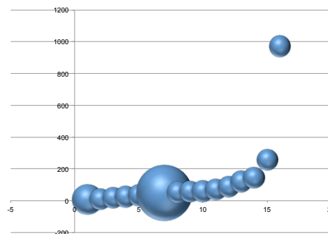
Figure 3: Sample size
